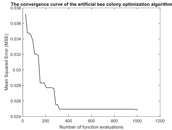
Figure 2: Convergence curve of the artificial bee colony optimization algorithm
