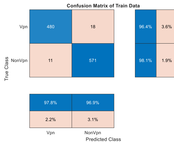
Figure 3: Confusion matrix of training data for the OSELM-Wavelet method
