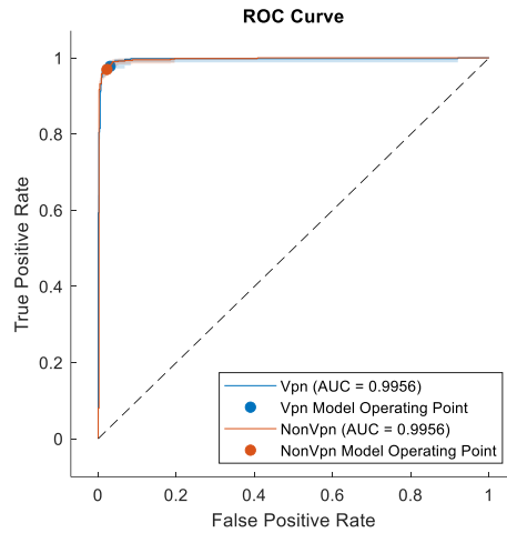
Figure 4 ROC curve for the OSELM-Wavelet method on test data
