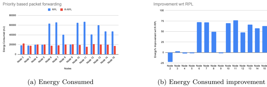
Fig. 8: Performance Metrics of Energy consumed in PPF
