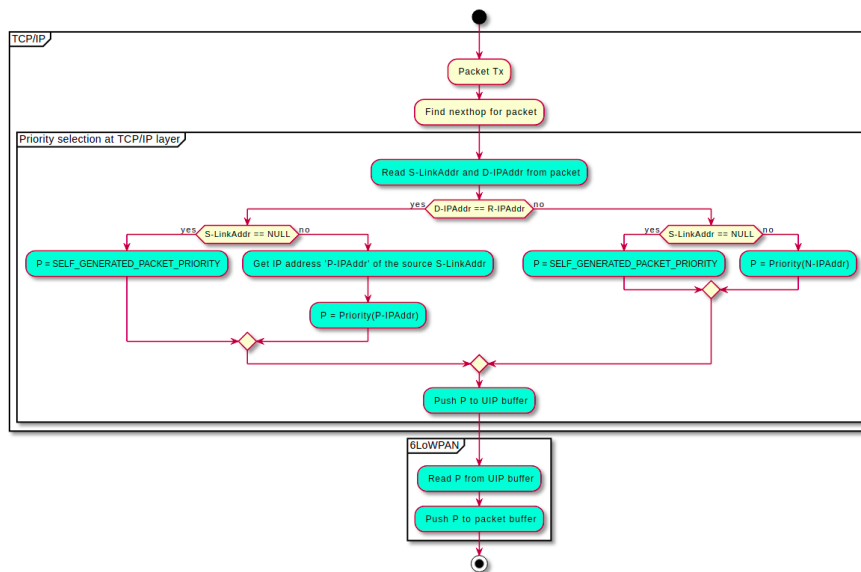
Fig. 4: Data-Plane Packet Prioritization With RPL Metric Advertisement
