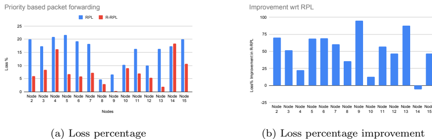
Fig. 7: Performance Metrics of Loss% in PPF
