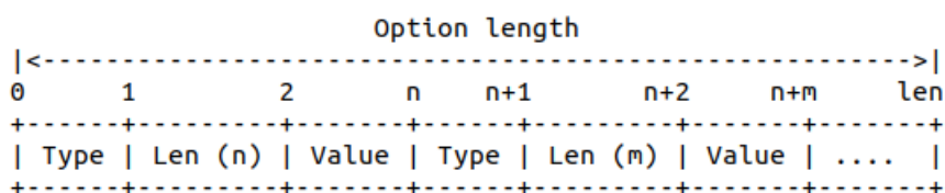
Fig. 3: Sub-option - Metric Advertisement message format
