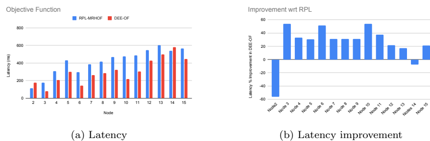
Fig. 12: Performance Metrics of Latency in R-RPL
