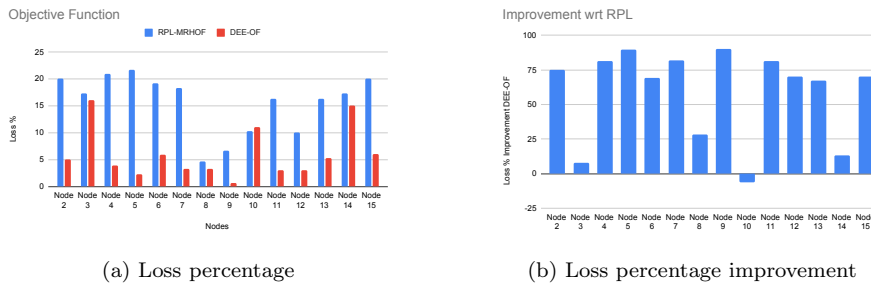
Fig. 10: Performance Metrics of Loss% in R-RPL
