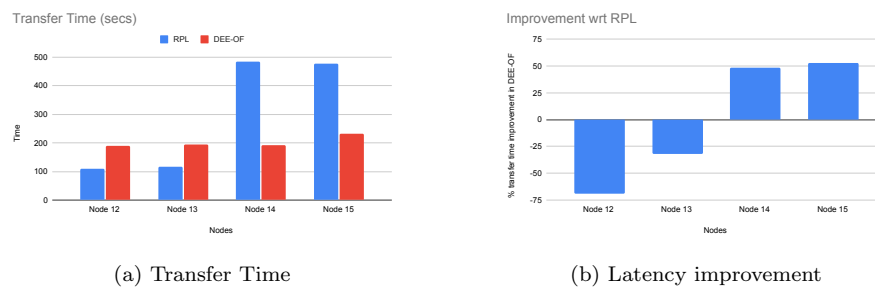
Fig. 13: Performance of Image transmission time
