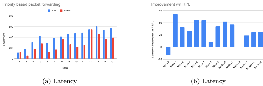
Fig. 9: Performance Metrics of Latency in PPF
