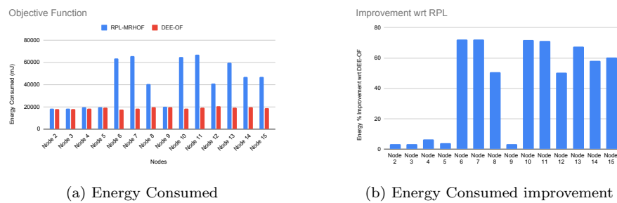
Fig. 11: Performance Metrics of Energy consumed in R-RPL
