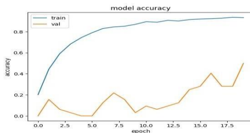
Figure 13. Graph for Model accuracies
