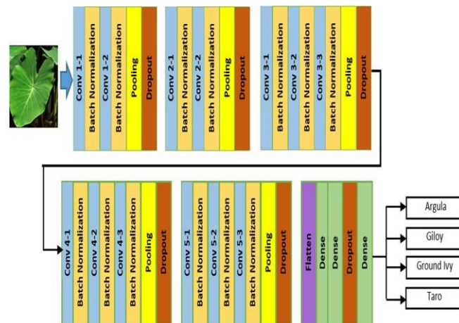
Figure 6. Different Layers used in the proposed methodology.
