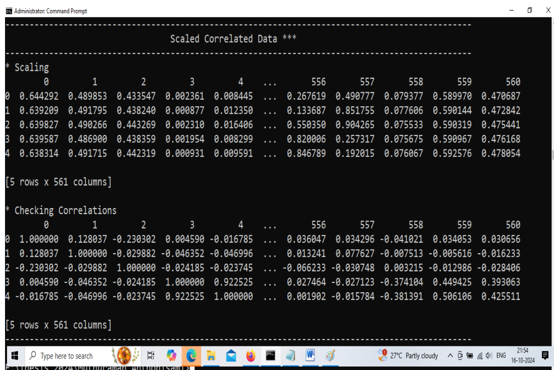
Figure 6. SRHADM's scaled-correlated Output
