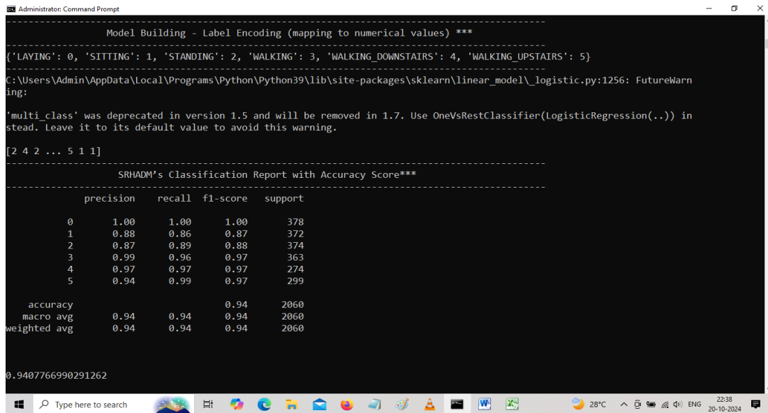
Figure 7. Modelling and accuracy outputs of SRHADM
