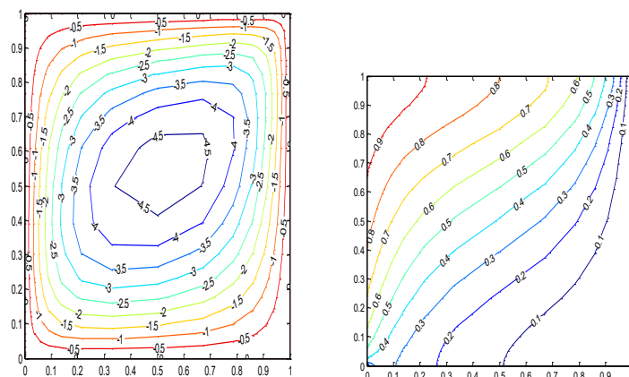
Fig: (7): Streamlines (Left) and Isotherms(Right) for A_r=1, R_d=1, \lambda=0.25
