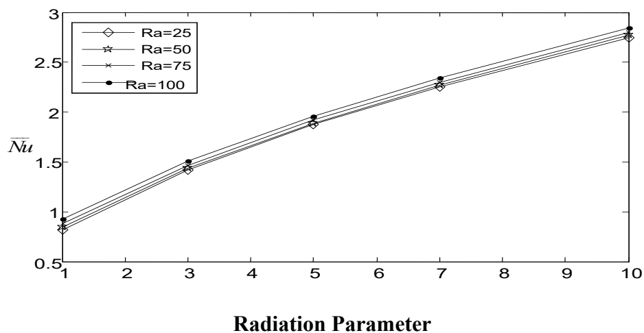
Fig: (14): \bar{Nu} Variations with R_d at hot surface for different values of Ra at Ar=1, \lambda=1
