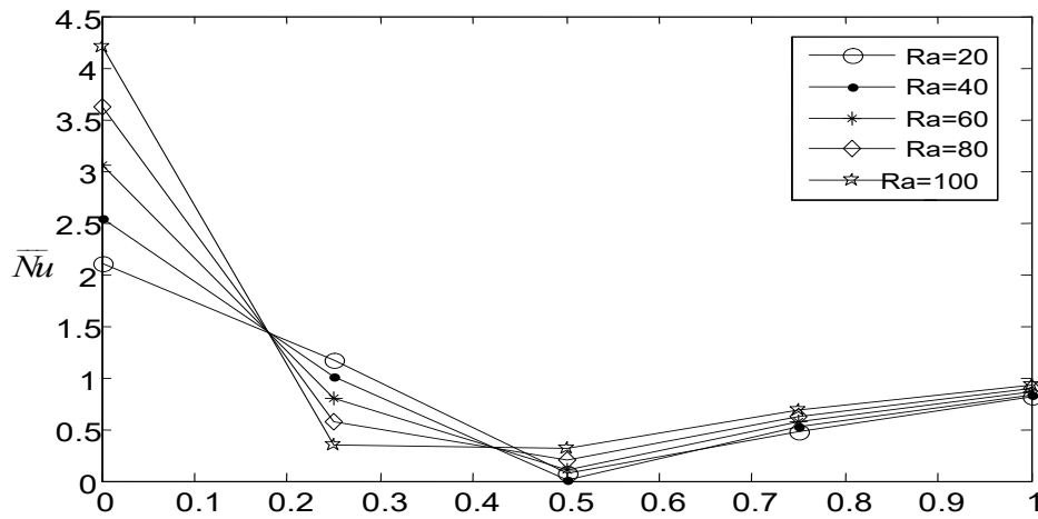
Fig: (13): \bar{Nu} Variations with \lambda at hot surface for different values of Ra at Ar=1, Rd=1
