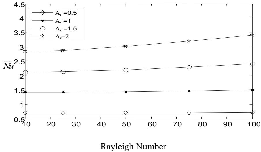
Fig: (11): \bar{Nu} Variations with Ra at hot surface for different values of A_r at \lambda = 1 , R_d = 3
