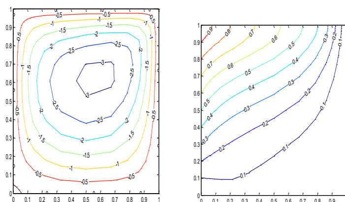
Fig: (6) : Streamlines (Left) and Isotherms (Right) for Ra=100 , Ar = 1 , R_d = 1
