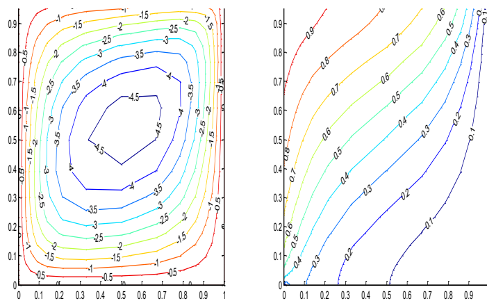
Fig: (2): Streamlines (Left) and Isotherms (Right) for Ra=100 , R_d=3 , \lambda=1 a) A_r=0.5 b) A_r=1 c) A_r=2
