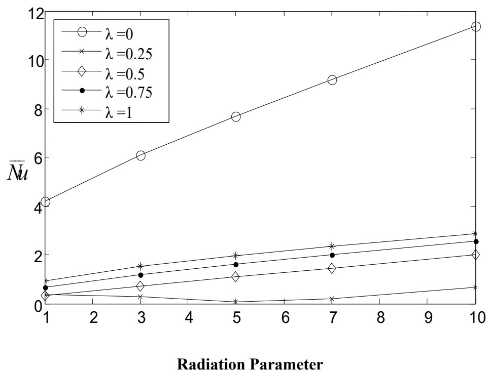
Fig: (10): \bar{Nu} Variations with R_d at hot surface for different values of \lambda at A_r=1, Ra=100
