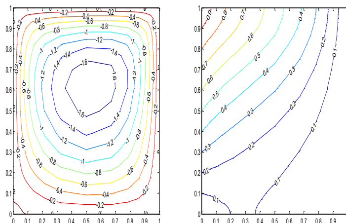
Fig: (5) : Streamlines (Left) and Isotherms(Right) for Ra=50 , Ar=1 , Rd=1
