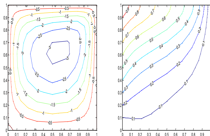
Fig. (8): Streamlines (Left) and Isotherms (Right) for Ar=1, Ra=1, \lambda=1 a) Ra=25 b) Ra=75 c) Ra=100
