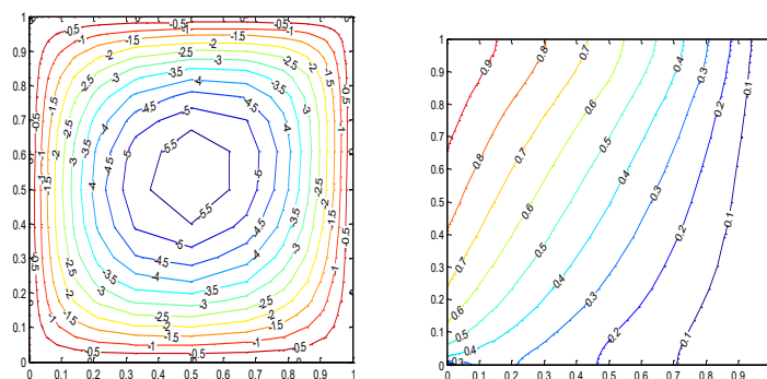
Fig: (3): Streamlines (Left) and Isotherms (Right) for Ra=100 , Ar=1 , \lambda=0.25
