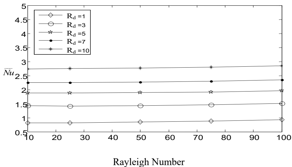
Fig: (12): \bar{Nu} Variations with Ra at hot surface for different values of R_d at \lambda = 1 , A_r = 1
