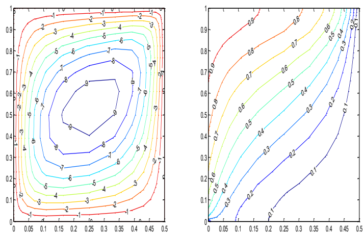
Fig: (1): Streamlines (Left) and Isotherms (Right) for Ra=100 , R_d=3 , \lambda=0.25
