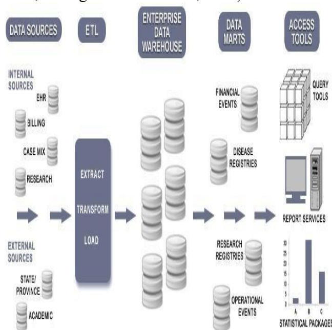
Figure1–Health Data Warehouse Architecture
