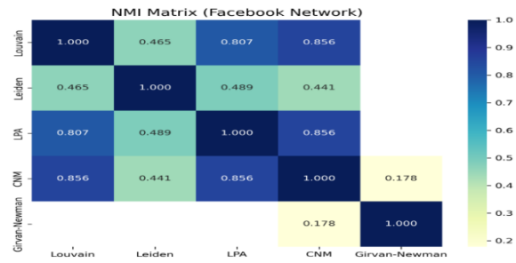
Fig. 7. The heatmap representation of the NMI score on Facebook’s Network
