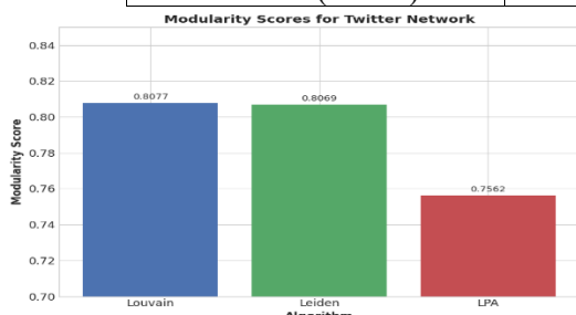
Fig. 4. Comparison of Modularity for different community detection algorithms on Twitter’s Network dataset
