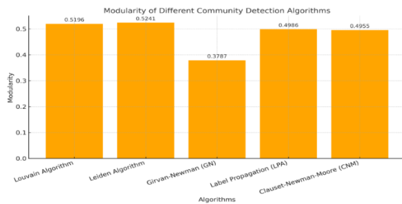
Fig. 2. Comparison of Modularity for different community detection algorithms on Dolphin’s Network dataset
