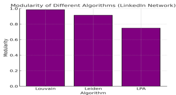
Fig. 8. Comparison of Modularity for different community detection algorithms on LinkedIn’s Network
