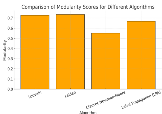
Fig. 10. Comparison of Modularity for different community detection algorithms on Citation's Network dataset
