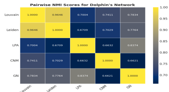
Fig. 3. The heatmap representation of the NMI score on Dolphin’s Network
