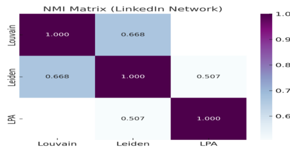
Fig. 9. The heatmap representation of the NMI score on LinkedIn’s Network
