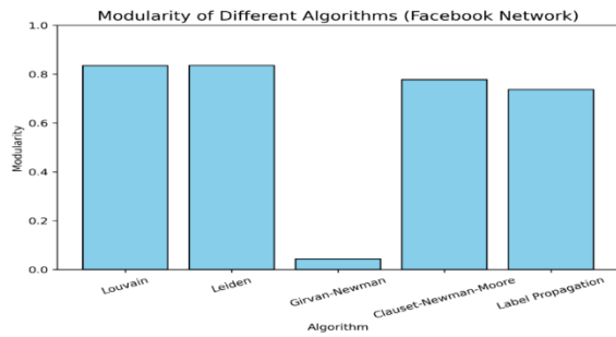
Fig. 6. Comparison of Modularity for different community detection algorithms on Facebook’s Network
