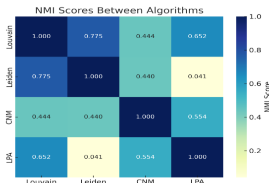
Fig. 11. The heatmap representation of the NMI score on Citation's Network
