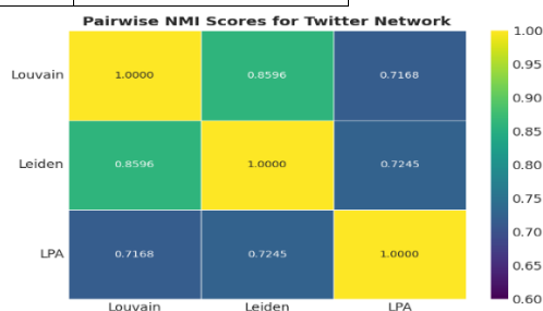
Fig. 5. The heatmap representation of the NMI score on Twitter’s Network
