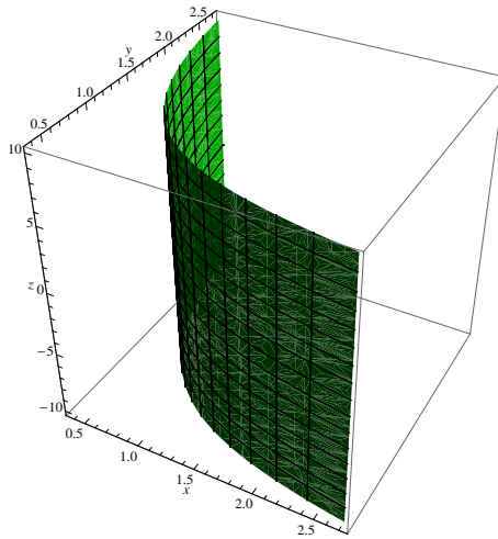
Figure 1: r(u, v) = (e^u, e^{-u}, v)
